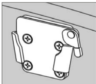
Quick Release Bracket (QR) The Quick Release Bracket is mounted into metal insert nuts and used with the IV Pole, Side Tray, and Oxygen Tank Holder.
