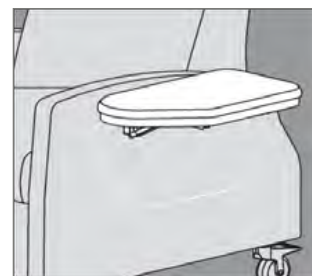
Padded Side Tray (PLFST) The PLFST is upholstered allowing patients to comfortably rest their arms during treatment. It measures 17" L x 10-5/8" W. When, in fold down position, tray extends 2-1/2" from side of arm. PLFST requires 1 yard of fabric.
